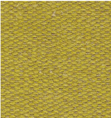
Tollan OWA03
